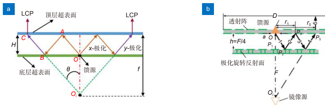
图2 无源折叠式透射阵超表面。(a)圆极化折叠式透射阵超表面 [42] ；(b)II型透射阵构型 [46] Fig. 2 Passive folded transmitarray metasurface. (a) Circularly-polarized folded transmitarray metasurface [42] ; (b) II-type folded transmitarray metasurface prototype [46]
