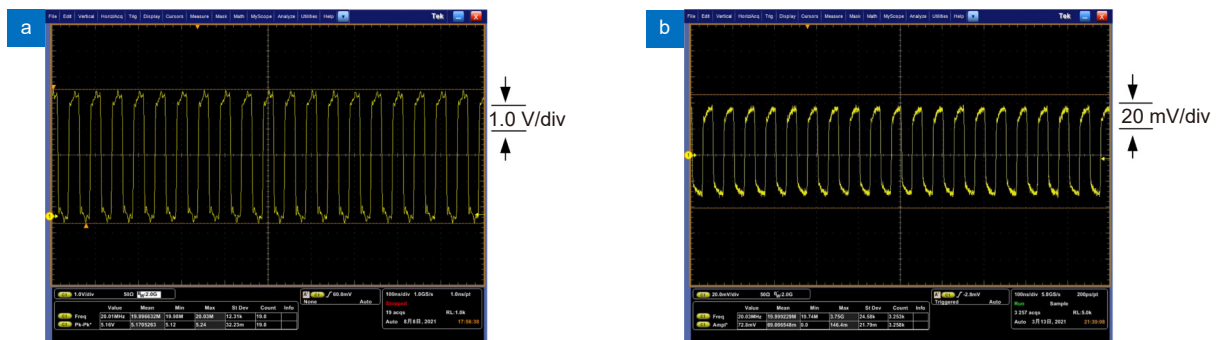
图 31 收发两端信号波形 [40] 。(a) 发射信号; (b) 接收信号 Fig. 31 Receive and transmit signal waveforms [40] . (a) Transmitting signal; (b) Receiving signal
