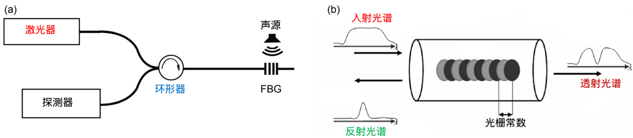
图 3 (a) 波长调制型光纤声传感器 [4] ; (b) 光纤布拉格光栅 [43] Fig. 3 (a) Optical fiber acoustic sensors with wavelength modulation [4] ; (b) Fiber Bragg grating [43]
