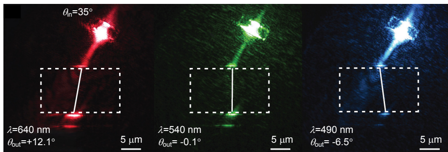
图 8 不同波长的光入射时, 光栅超表面折射的实验结果. 光栅周期 150 nm, 宽度 90 nm, 高度 80 nm [75] . Fig. 8 Image of SPPs refraction at different wavelengths. The grating period is 150 nm, the width is 90 nm and the height is 80 nm [75] .
